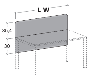
Pannello divisori con minigonna Sp. 1,8 cm Partition screen with modesty panel 1,8cm-thick
